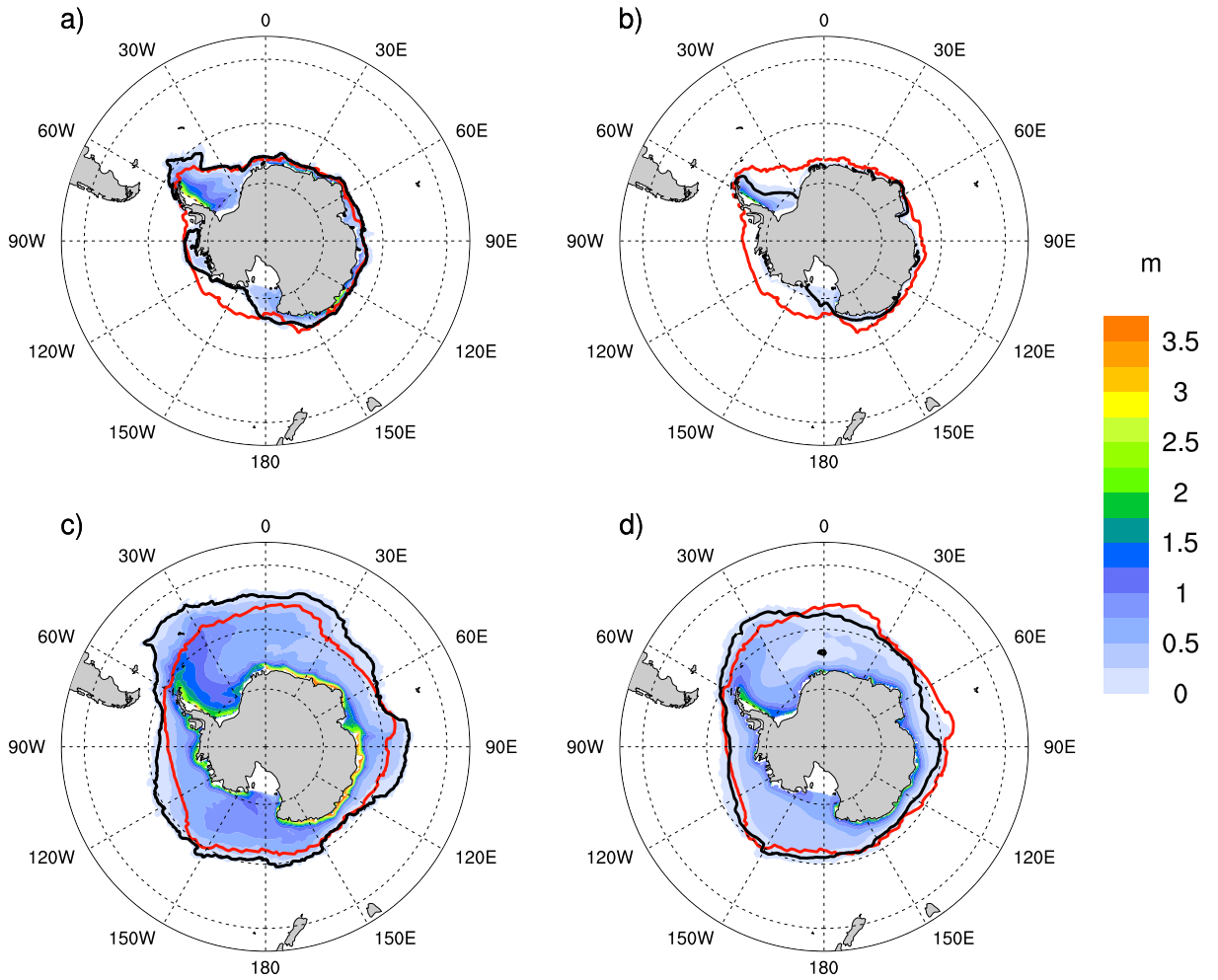
Figure 9: Sea ice SH 1861-1865
