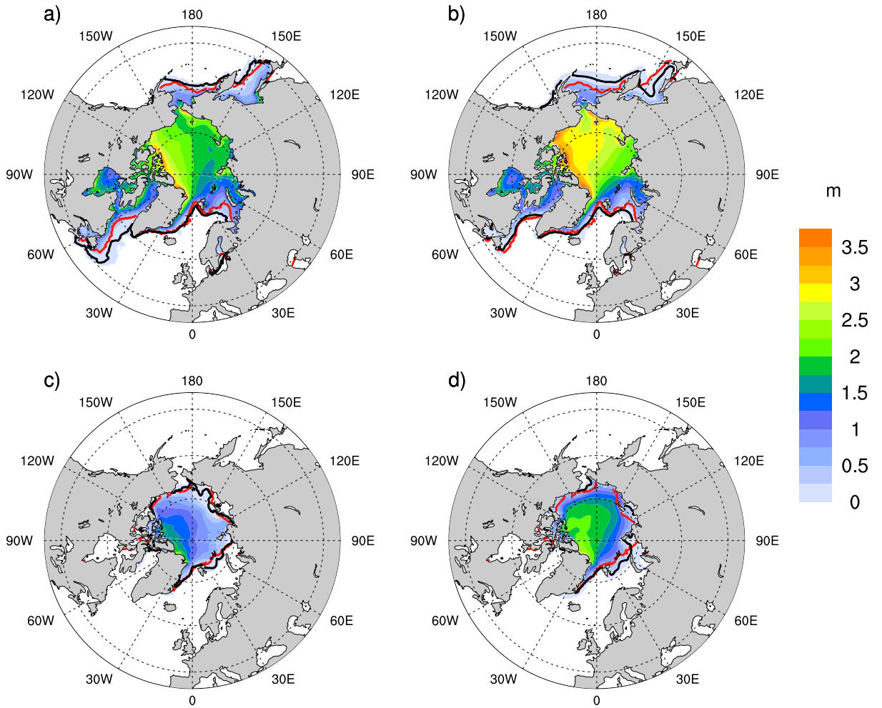
Figure 8: Sea ice NH 1866-1870
