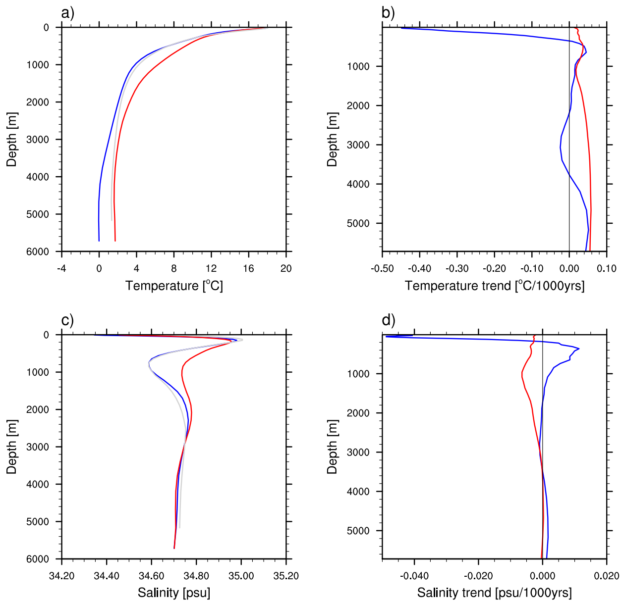
Figure 5: Vert. profiles 1861-1865
