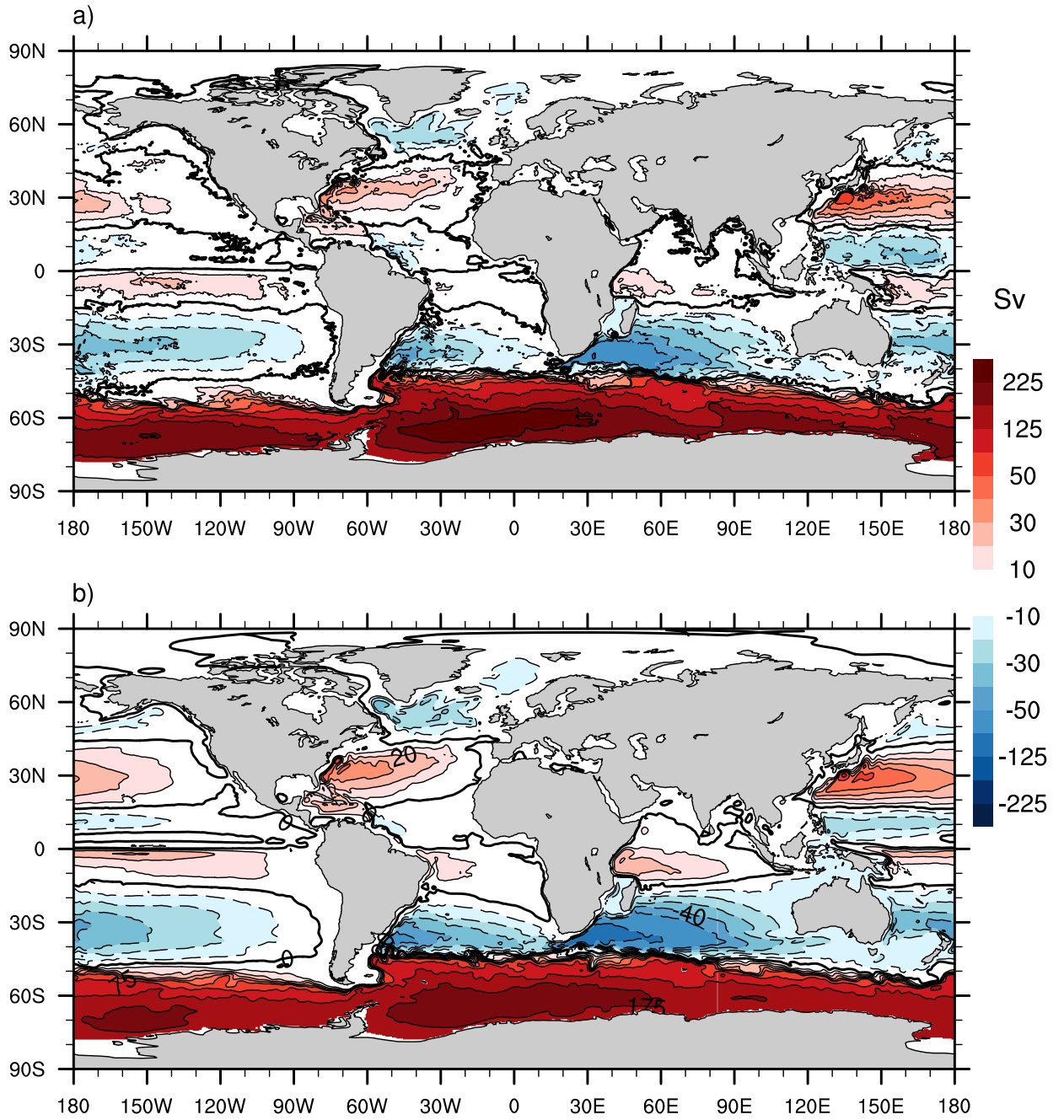
Figure 13: Barotropic stream function 1861-1865
