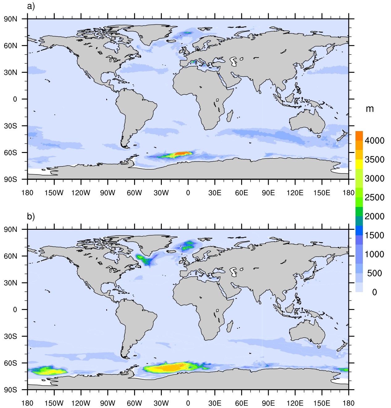
Figure 12: Max. mixed layer 1866-1870
