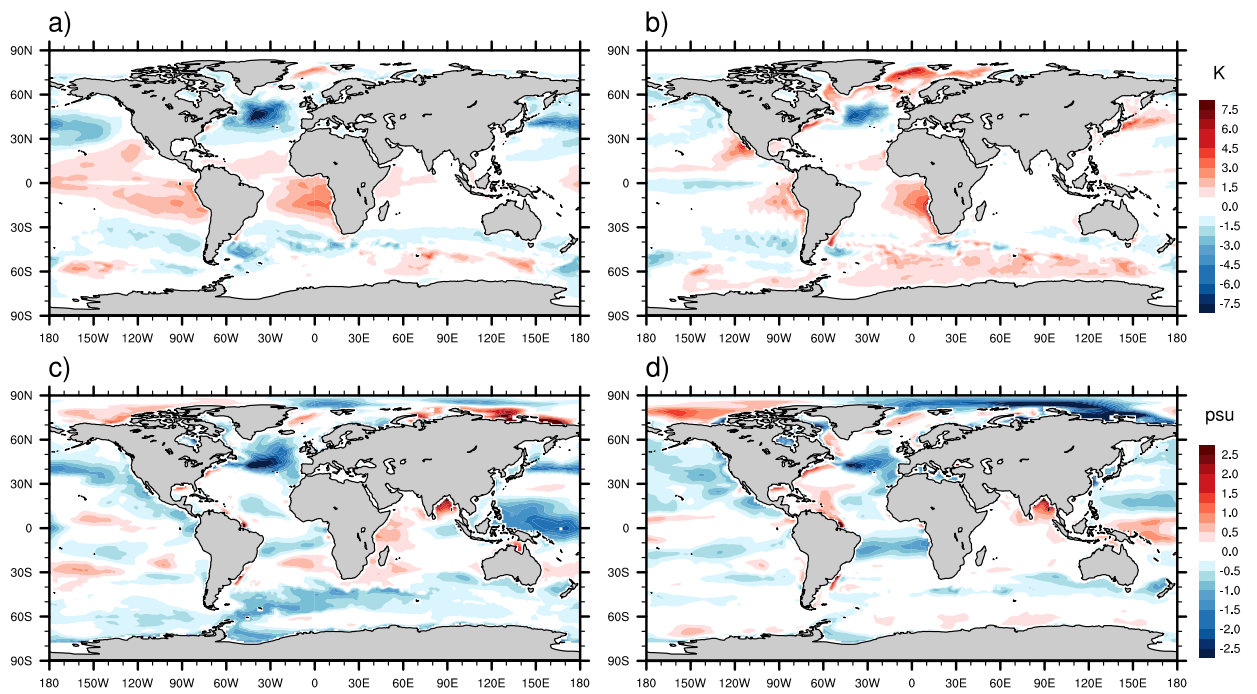
Figure 3: Surface biases 1861-1865
