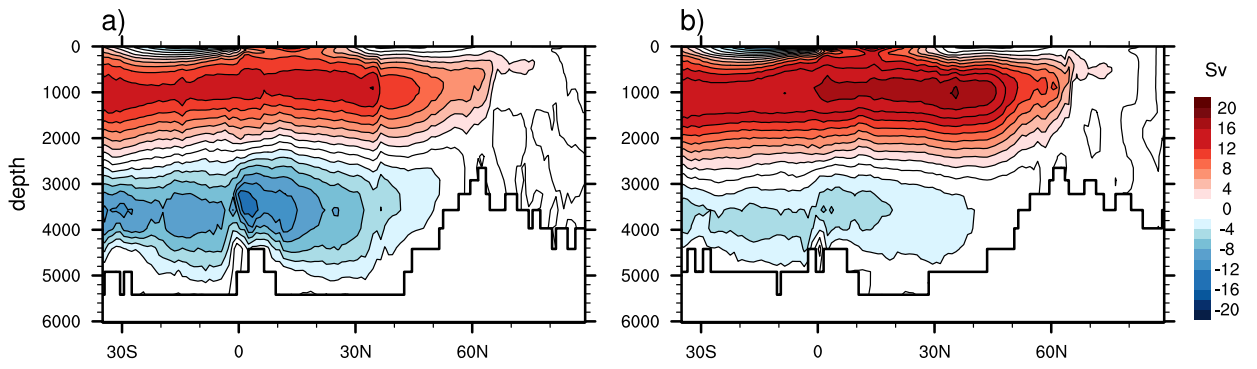
Figure 1: MOC 1861-1865
