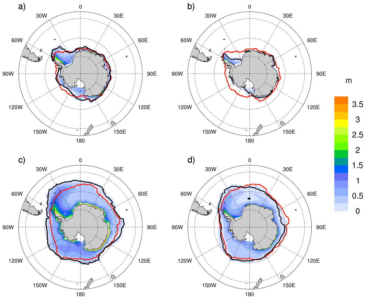
Figure 10: Sea ice SH 1866-1870
