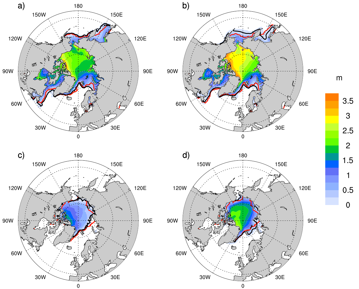
Figure 7: Sea ice NH 1861-1865
