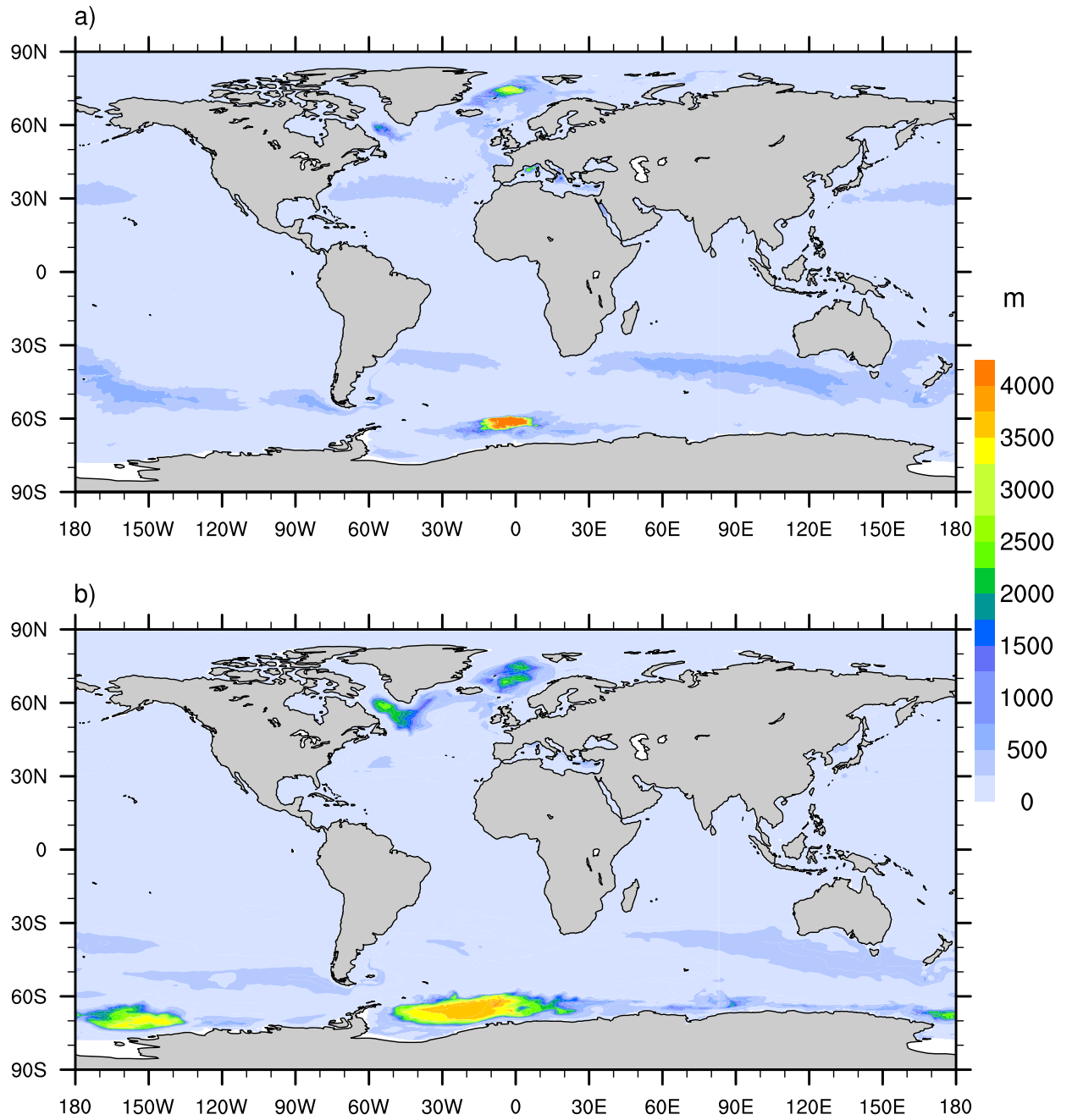
Figure 11: Max. mixed layer 1861-1865
