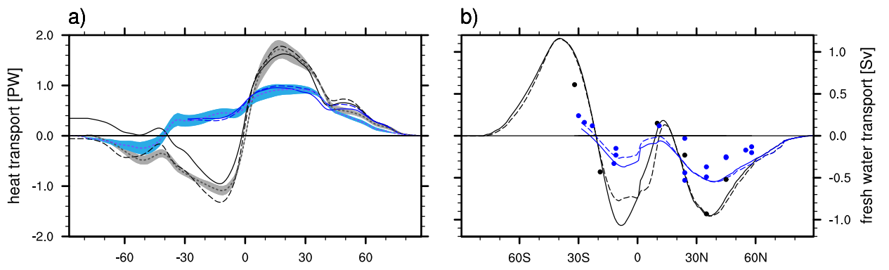
Figure 6: Heat and Fresh water transports 1861-1865
