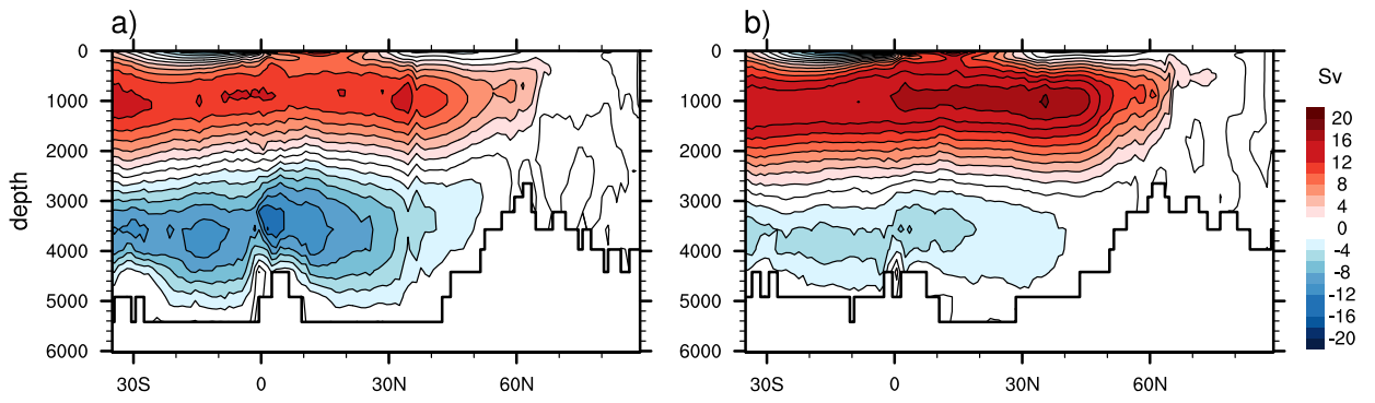
Figure 2: MOC 1866-1870
