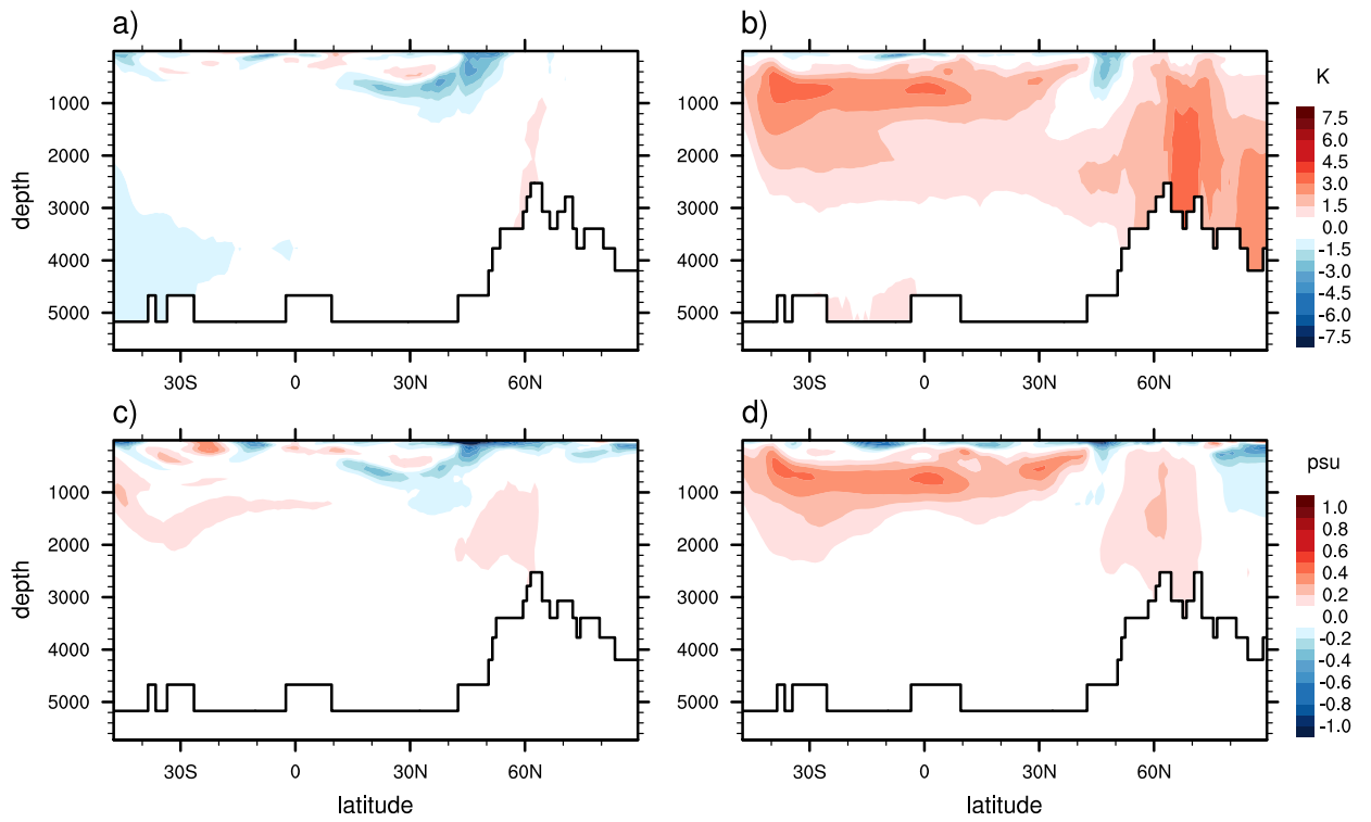
Figure 4: Zon. mean biases 1861-1865, Atlantic
